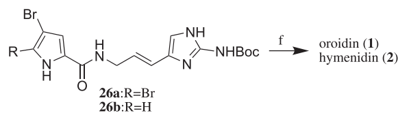
Scheme 4. Total synthesis of oroidin ( 1 ) and hymenidin ( 2 ). Reagents and conditions: (a) N -(2-bromoethyl)phthalimide, \text{K}_2\text{CO}_3 /acetone, reflux, 3 h; (b) m -CPBA, \text{NaHCO}_3/\text{CH}_2\text{Cl}_2 , rt, overnight, 79% (two steps from 22 ); (c) 21a (1.5 equiv), NaHMDS/THF, –78 °C, 30 min, 69%; (d) \text{H}_2\text{NNH}_2/\text{EtOH} , 50 °C, 2 h, 92%; (e) 4,5-dibromo-2-trichloroacetylpyrrole or 4-bromo-2-trichloroacetylpyrrole, \text{Na}_2\text{CO}_3/\text{DMF} , rt, overnight, 79% for 26a , 83% for 26b ; (f) 20% HCl/EtOH, rt, 1 h, 92% for 1 , 99% for 2 .
