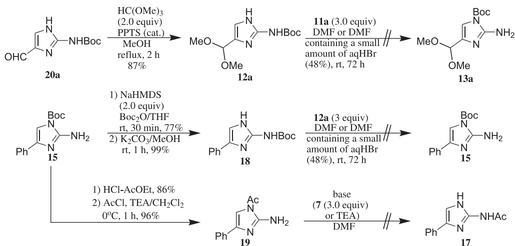
Scheme 2. Reactions of tert -butyl 4-dimethoxymethyl-1 H -imidazol-2-ylcarbamate ( 12a ), tert -butyl 4-phenyl-1 H -imidazol-2-ylcarbamate ( 18 ) and 1-(2-amino-4-phenyl-1 H -imidazol-1-yl)ethanone ( 19 ).
