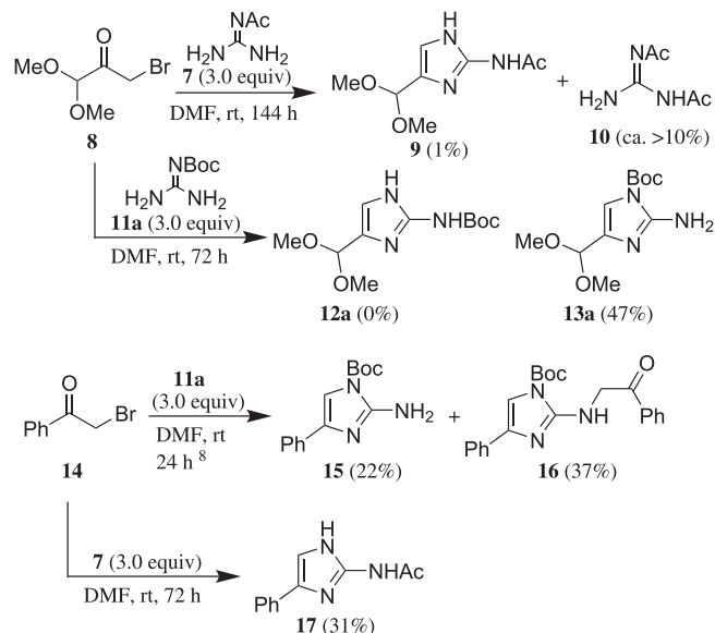
Scheme 1. Reactions of the acylguanidine derivatives ( 7 and 11a ) with 3-bromo-1,1-dimethoxypropan-2-one ( 8 ) and phenacyl bromide ( 14 ).
